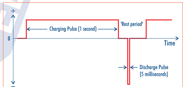
Fig.3: The type of charging current waveform used in pulse chargers, and especially those using discharge-pulse 'burping'.
