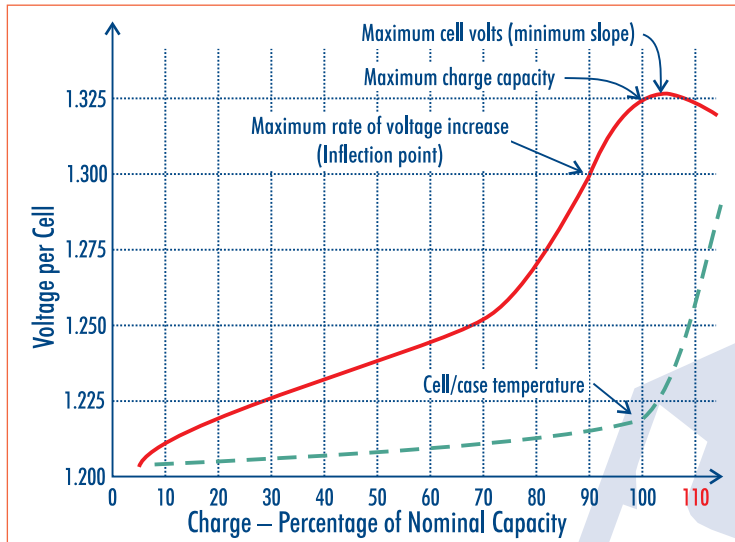
Fig.2: How the terminal voltage of a typical NiCad cell (and also its temperature) tends to vary during charging. Both the inflection point and the voltage peak are used for end-of-charge detection in high-end chargers.
